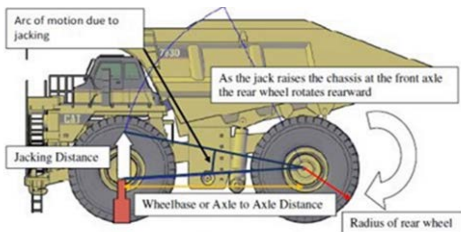
Image 4: Typical movement when jacking large vehicles
