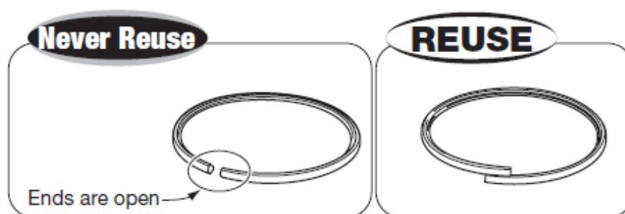
Image 5: Lock ring suitability (Source: Topy 2008.08)
